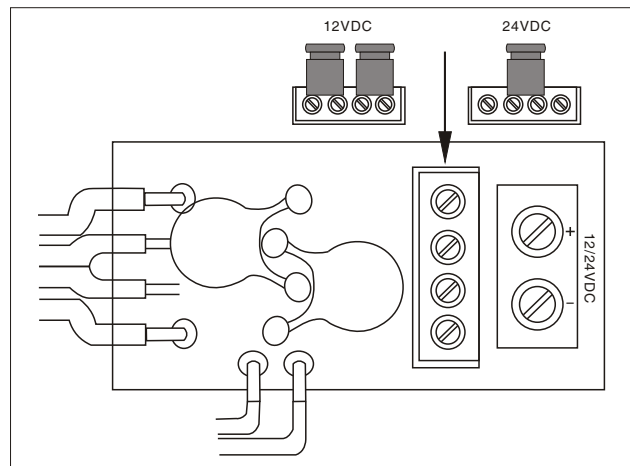
Wiring Diagram
