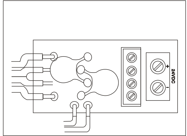
Wiring Instructions
